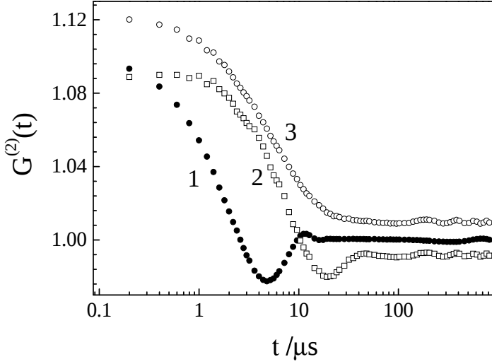
Figure 6.7: Autocorrelation function of 4O.8 membranes of different thickness measured at q_z = 2.2 \text{ nm}^{-1} : 0.3 \mu\text{m} (filled circles), 4.0 \mu\text{m} (squares) and 7.0 \mu\text{m} (open circles). Curves 2 and 3 are shifted by \pm 0.01 for clarity.
