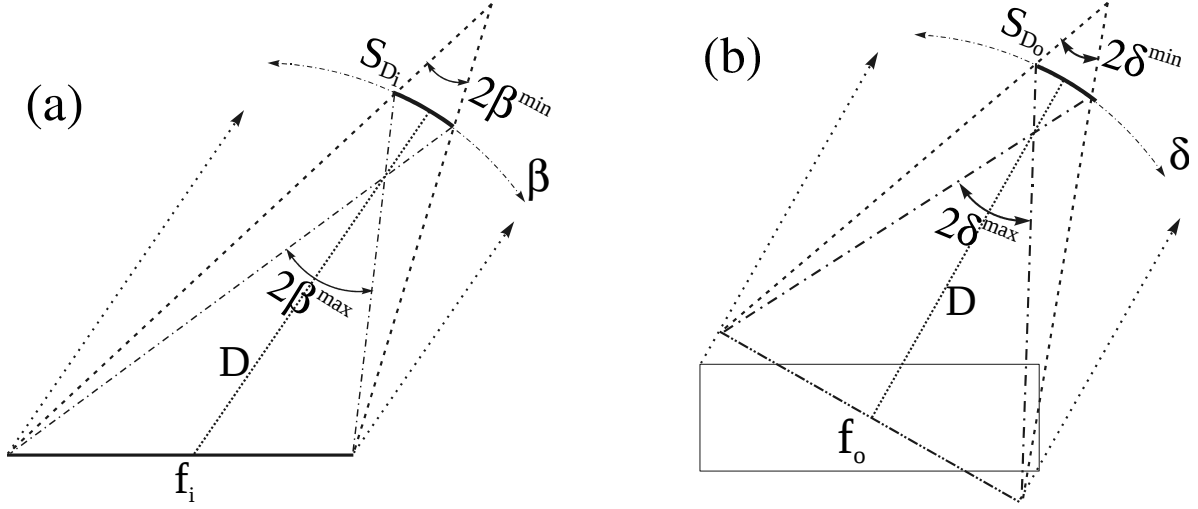
Figure 3.11: Acceptance angles of the detector in the scattering plane: 2\beta^{\min} and 2\beta^{\max} (a), and out of the scattering plane: 2\delta^{\min} and 2\delta^{\max} (b). The acceptance angles of the detector entrance are defined by the detector slits S_{D_{i,o}} , the footprint f_{i,o} on the sample and the distance D from the detector to the center of the diffractometer.
