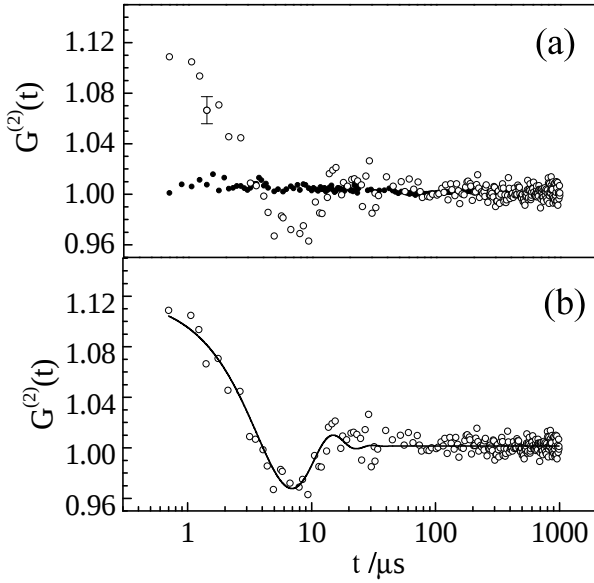
Figure 6.4: Autocorrelation function at q_z = 2.2 \text{ nm}^{-1} for a 95-layer membrane (thickness 0.27 \mu\text{m} ) in the SmA phase at 50.1^\circ \text{C} .
